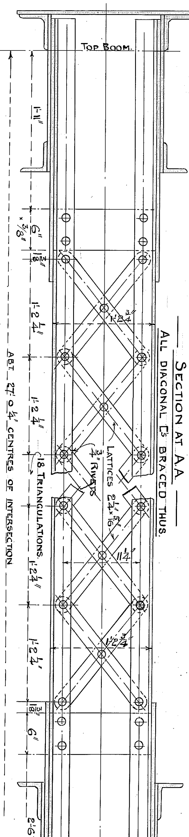
ALL CONNECTIONS TO BE MADE ABOARD BY MEANS OF TURNED BOLTS
