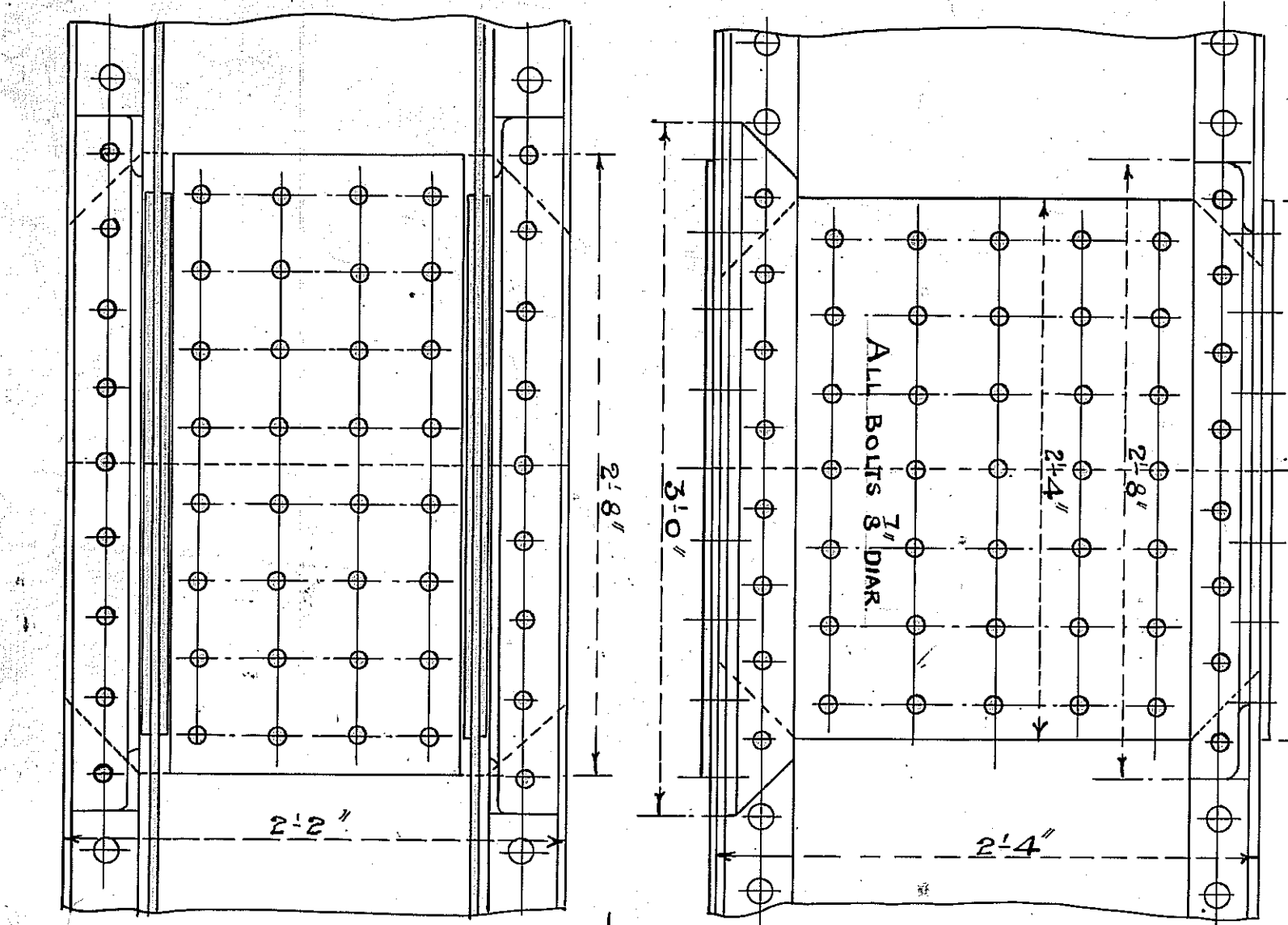
DETAIL OF JOINT IN BOTTOM BOOM
