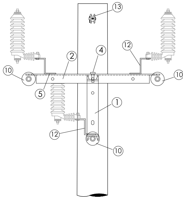
VISTA FRONTAL
