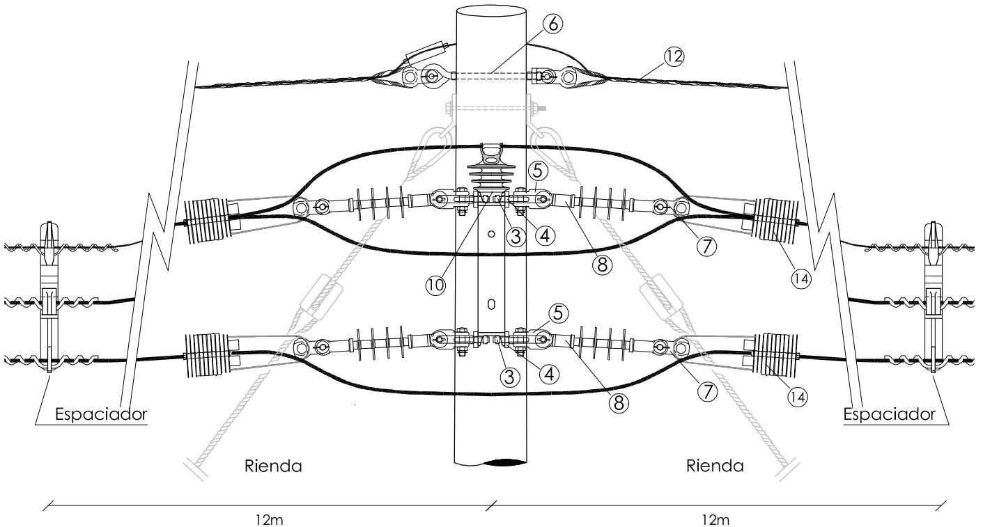
VISTA FRONTAL
